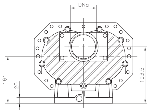
Non-drive end view / Vista lato opposto comando
